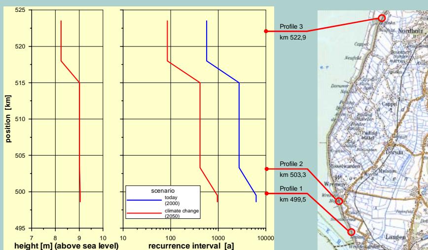
Figure 2: Recurrence interval of failure (wave overtopping) for three dike profiles at the coastline north of Bremerhaven calculated without and with water level rise of 55 cm
